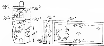
Figs. 5031-32. STOP-PLATE.
